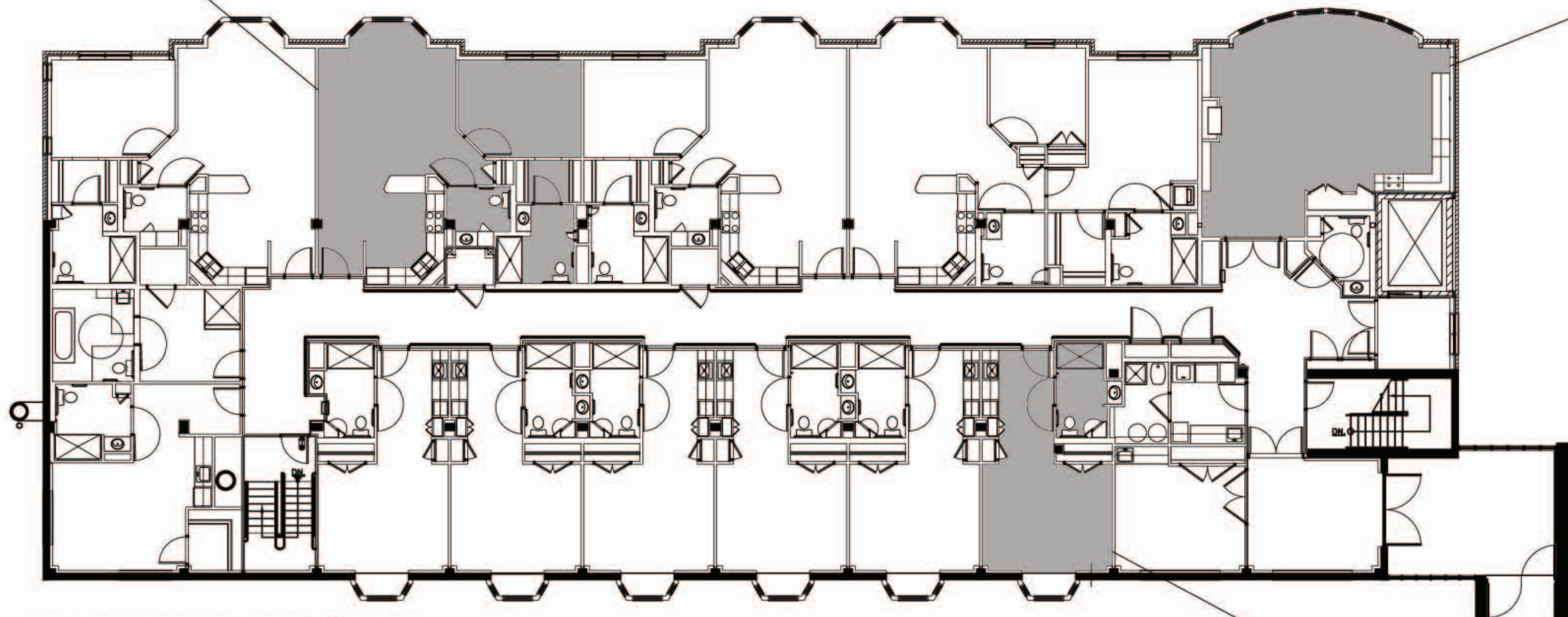
WEST HALL KEY PLAN
